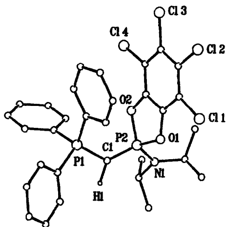
figure 1. Structure of the cation in 3
