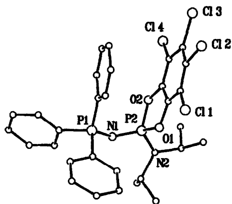
Structure of the cation in 8
